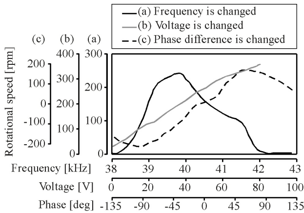
Fig. 3 Motor characteristics
