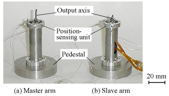
Fig. 5 Master and slave arms for active endoscope
