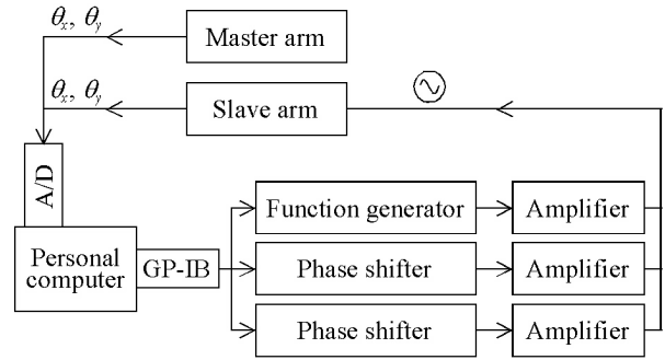
Fig. 9 Master-slave system
