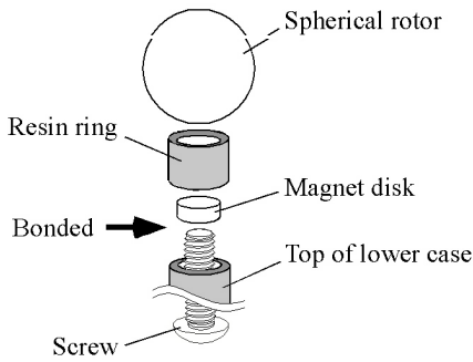
Fig. 8 Rotor/stator contact unit
