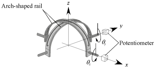
Fig. 7 Position sensing unit
